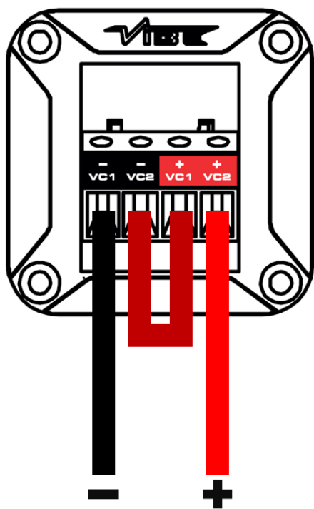
SERIES ( 4\Omega IMPEDANCE)
