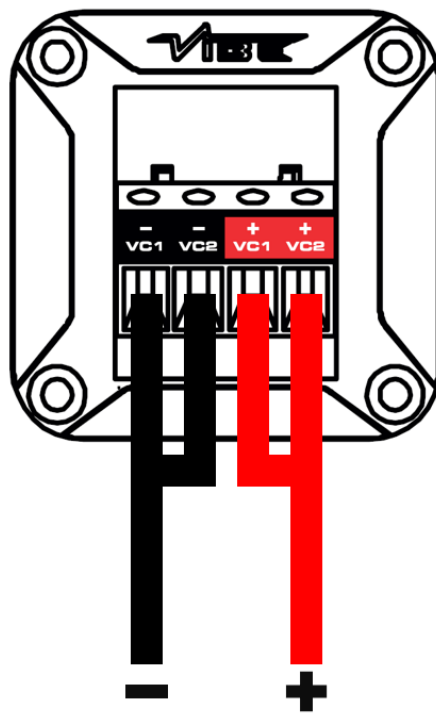
PARALLEL ( 1\Omega IMPEDANCE)
